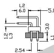
R2 TYPE
