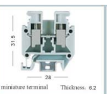
MBK 5/E-Z
