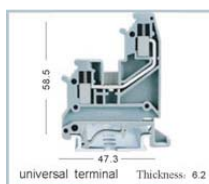
UK5-RETURN
