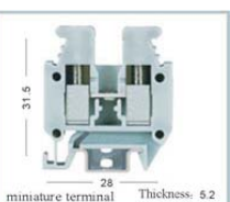
MBK3/E-Z
