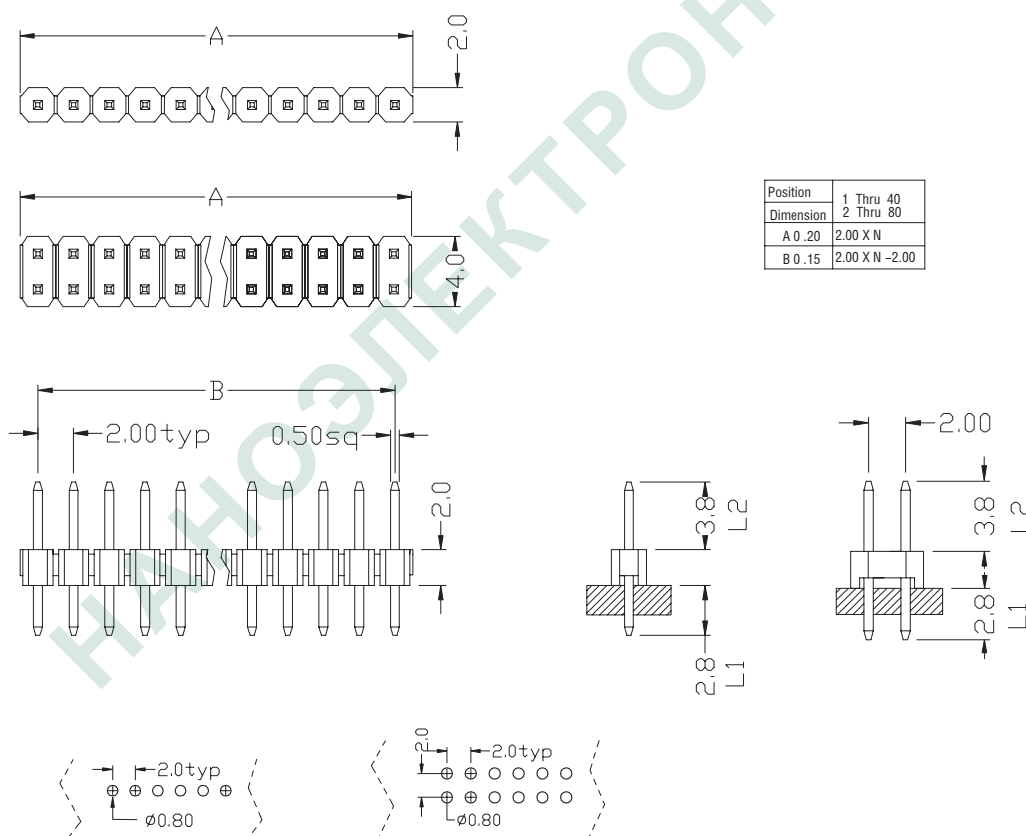
P. C. B Layout
