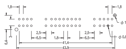
P.C.B. HOLE DETAIL
