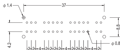
P.C.B. HOLE DETAIL
