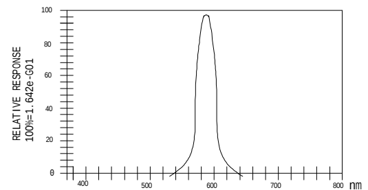
Luminous Spectrum ( T_a=25^{\circ}\text{C} ) SPECTRAL RADIANCE
